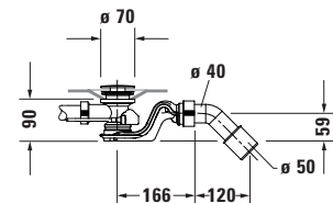
Siphon for whirltub # 760432
