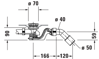
Siphon for bathtub # 700433
