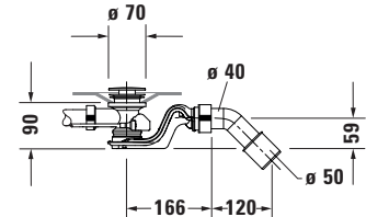
Siphon for bathtub # 700432
