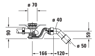
Siphon for whirltub # 760433
