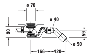
Siphon for whirltub # 760431
