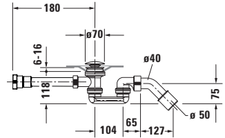
Siphon for bathtub # 700434
