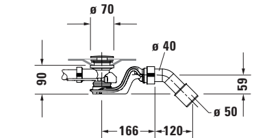
Siphon for bathtub # 700431
